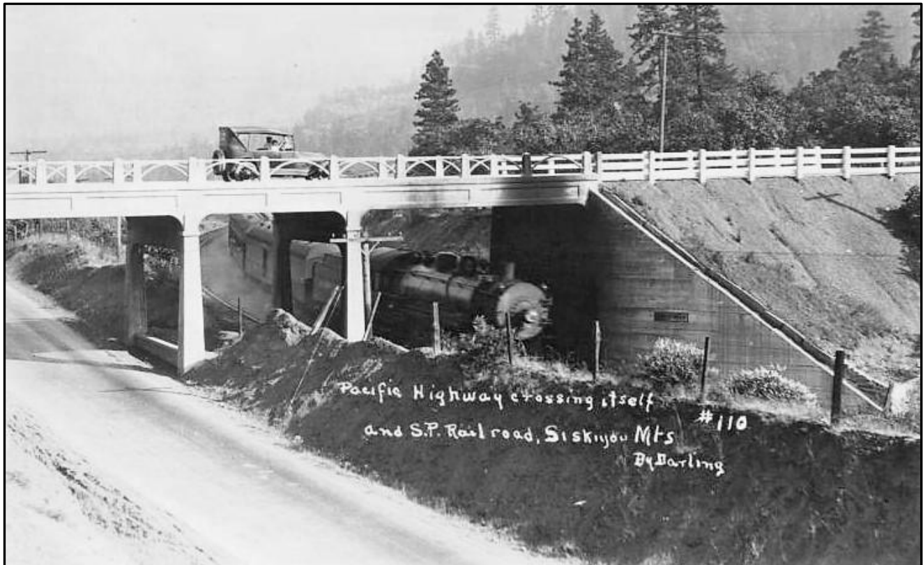
Built in 1914, the Steinman overcrossing on the Pacific Highway crosses over itself and the Southern Pacific Railroad. The historic crossing is still in use today and is part of Oregon Route 273 in southwest Oregon, near Ashland.
